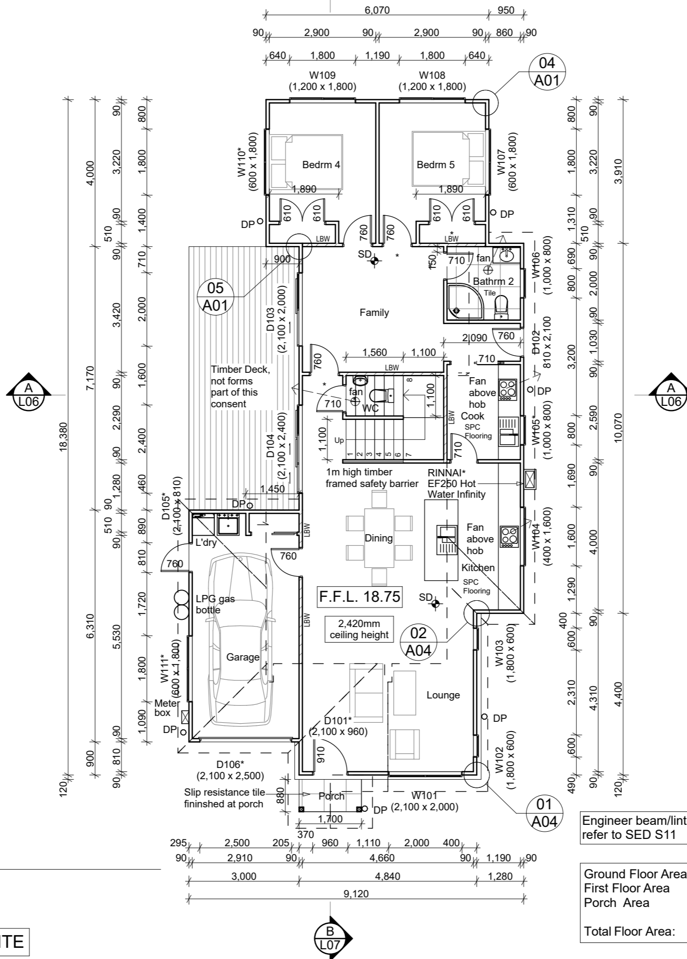
1. Ground Floor Plan 1:100
